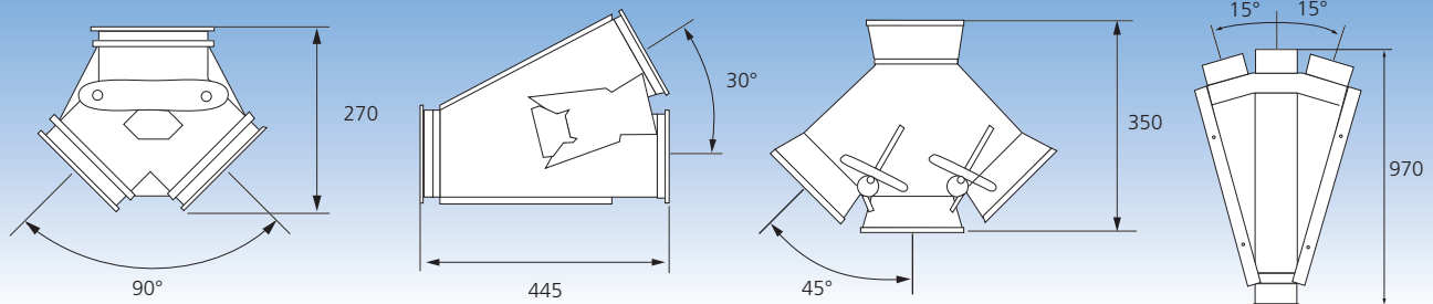
Trouser divertes, 45°, grey
