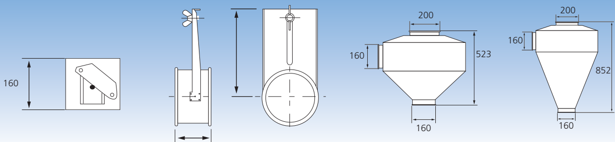
Throttle valves with spring, grey
