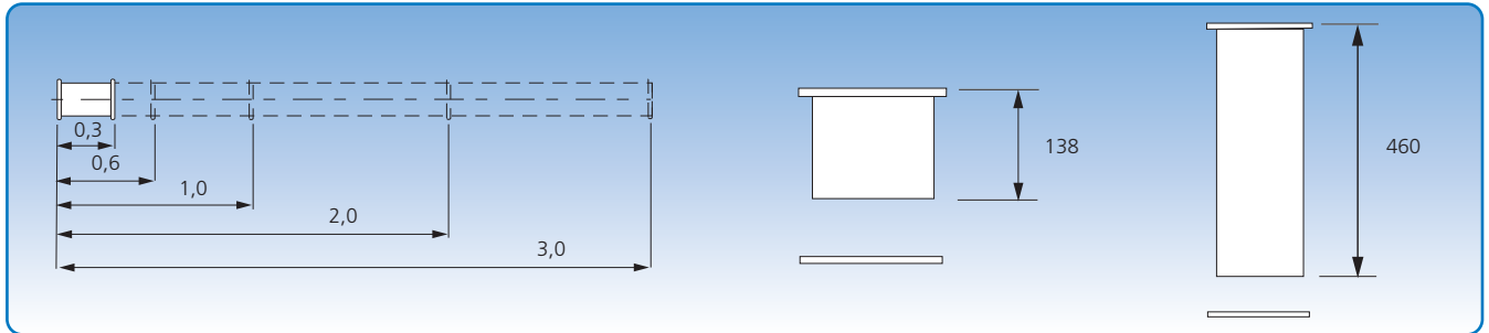
JK-6" duct system, galvanised
